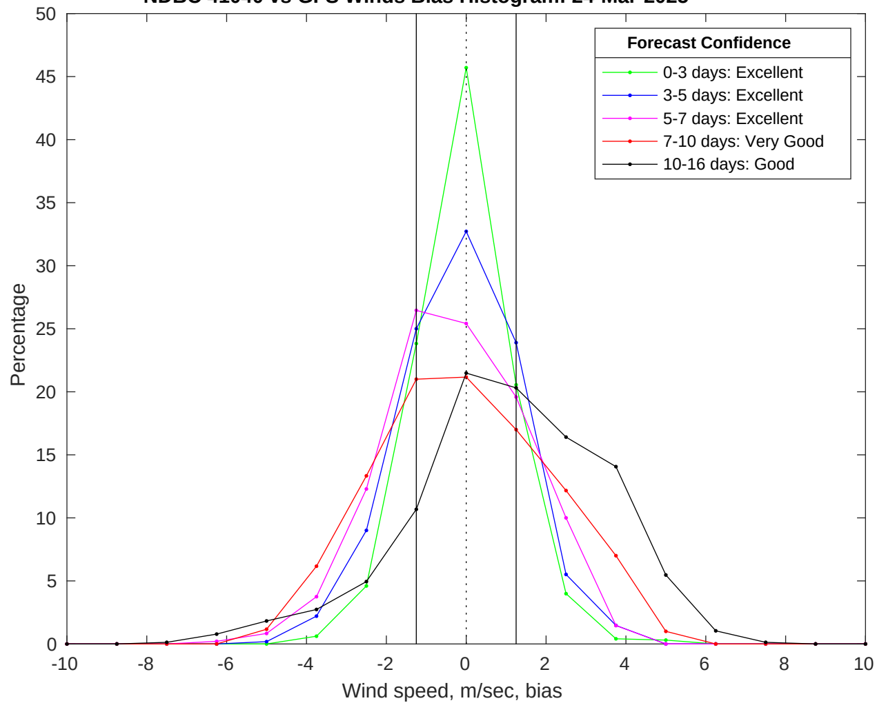
NDBC 41040 vs GFS Winds Bias Histogram: 24-Mar-2025
