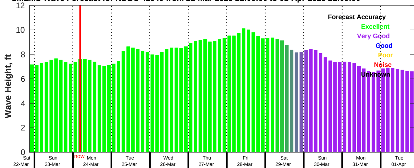
CMEMS Wave Forecast for NDBC 41040 from 22-Mar-2025 21:00:00 to 01-Apr-2025 21:00:00
