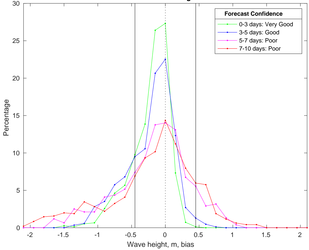
NDBC 42019 vs CMEMS Waves Bias Histogram: 24-Mar-2025
