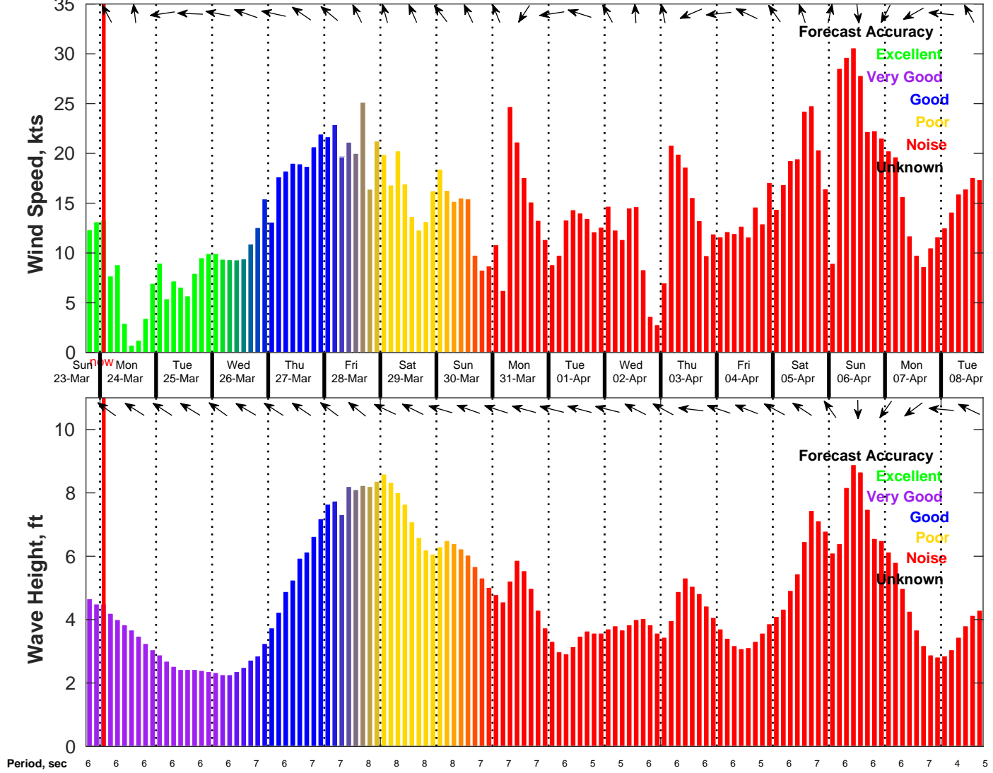
Wind & Wave Forecast for NDBC 42019 from 23-Mar-2025 18:00:00 to 08-Apr-2025 18:00:00
