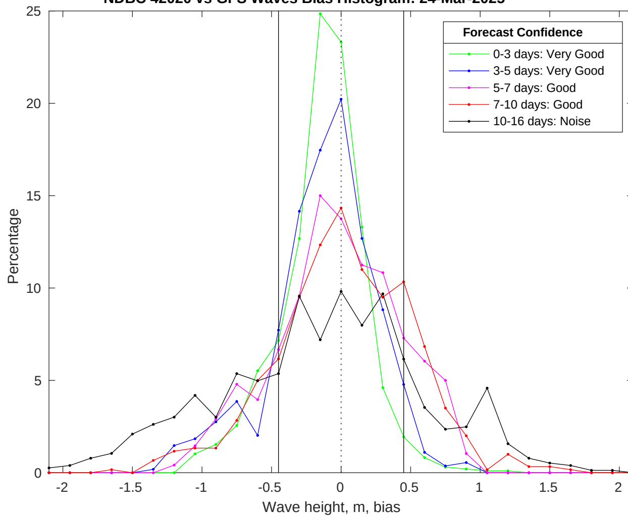
NDBC 42020 vs GFS Waves Bias Histogram: 24-Mar-2025
