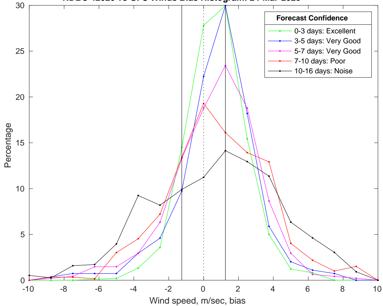
NDBC 42020 vs GFS Winds Bias Histogram: 24-Mar-2025
