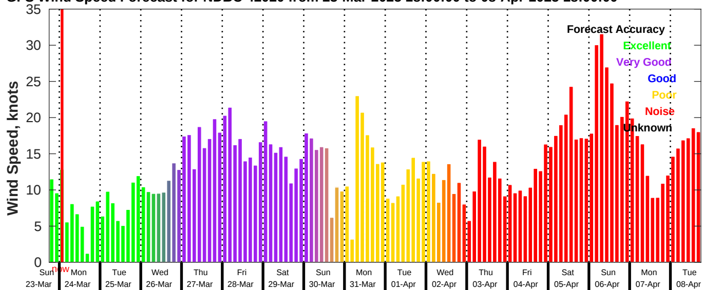
GFS Wind Speed Forecast for NDBC 42020 from 23-Mar-2025 18:00:00 to 08-Apr-2025 18:00:00
