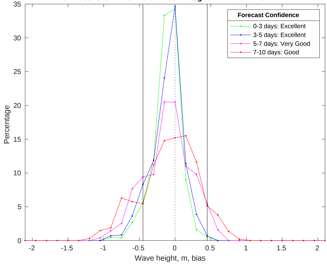
NDBC 42035 vs CMEMS Waves Bias Histogram: 24-Mar-2025
