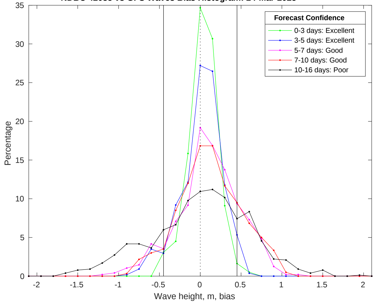
NDBC 42035 vs GFS Waves Bias Histogram: 24-Mar-2025
