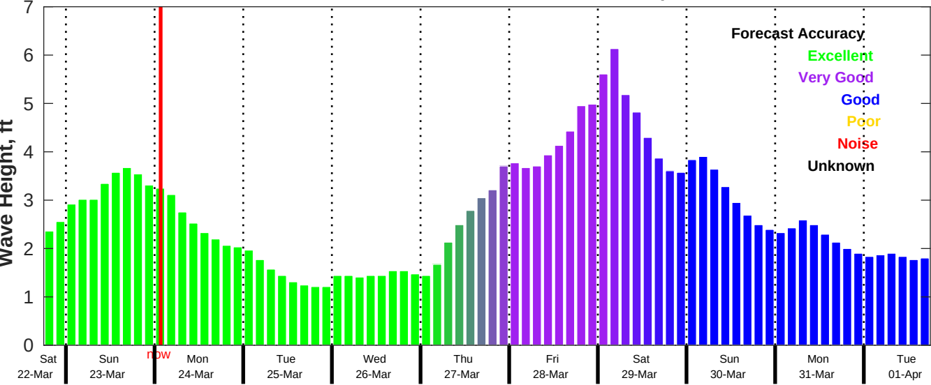
CMEMS Wave Forecast for NDBC 42035 from 22-Mar-2025 18:00:00 to 01-Apr-2025 18:00:00
