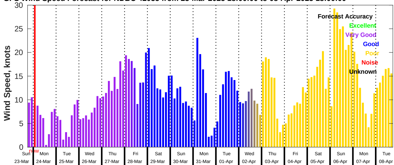
GFS Wind Speed Forecast for NDBC 42035 from 23-Mar-2025 18:00:00 to 08-Apr-2025 18:00:00
