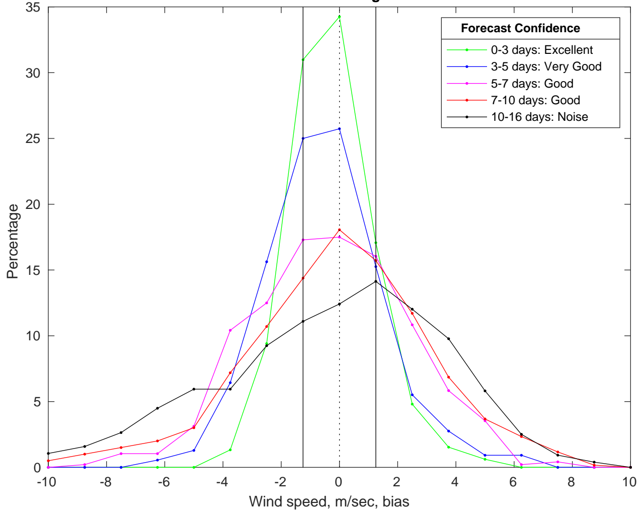
NDBC 42036 vs GFS Winds Bias Histogram: 24-Mar-2025
