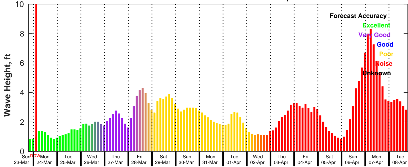
GFS Wave Forecast for NDBC 42036 from 23-Mar-2025 19:00:00 to 08-Apr-2025 19:00:00
