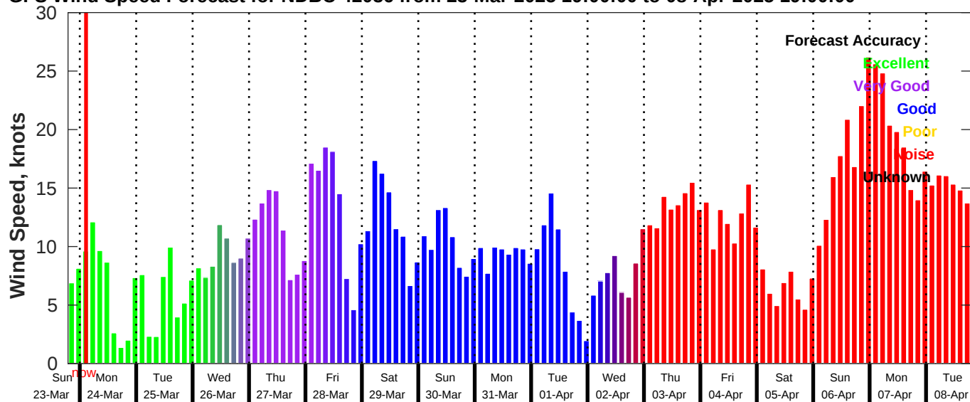
GFS Wind Speed Forecast for NDBC 42036 from 23-Mar-2025 19:00:00 to 08-Apr-2025 19:00:00
