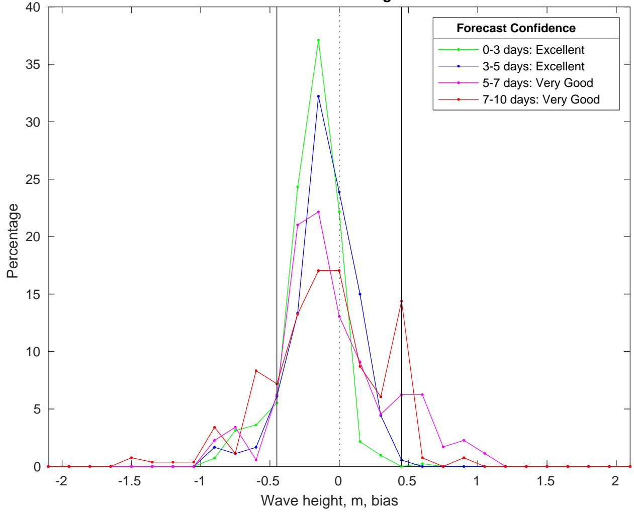
NDBC 42040 vs CMEMS Waves Bias Histogram: 24-Mar-2025
