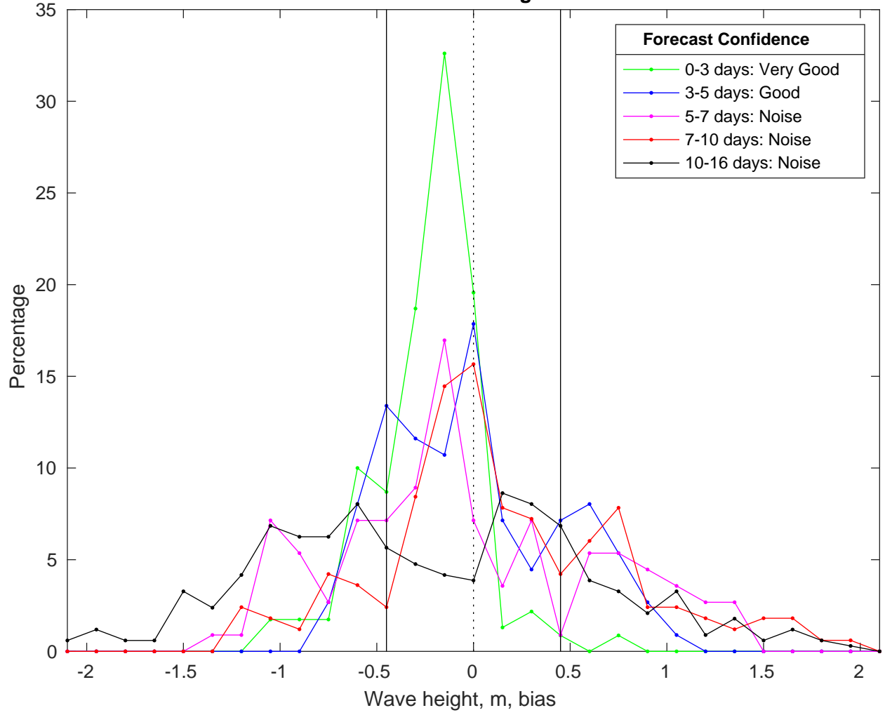
NDBC 42040 vs GFS Waves Bias Histogram: 24-Mar-2025
