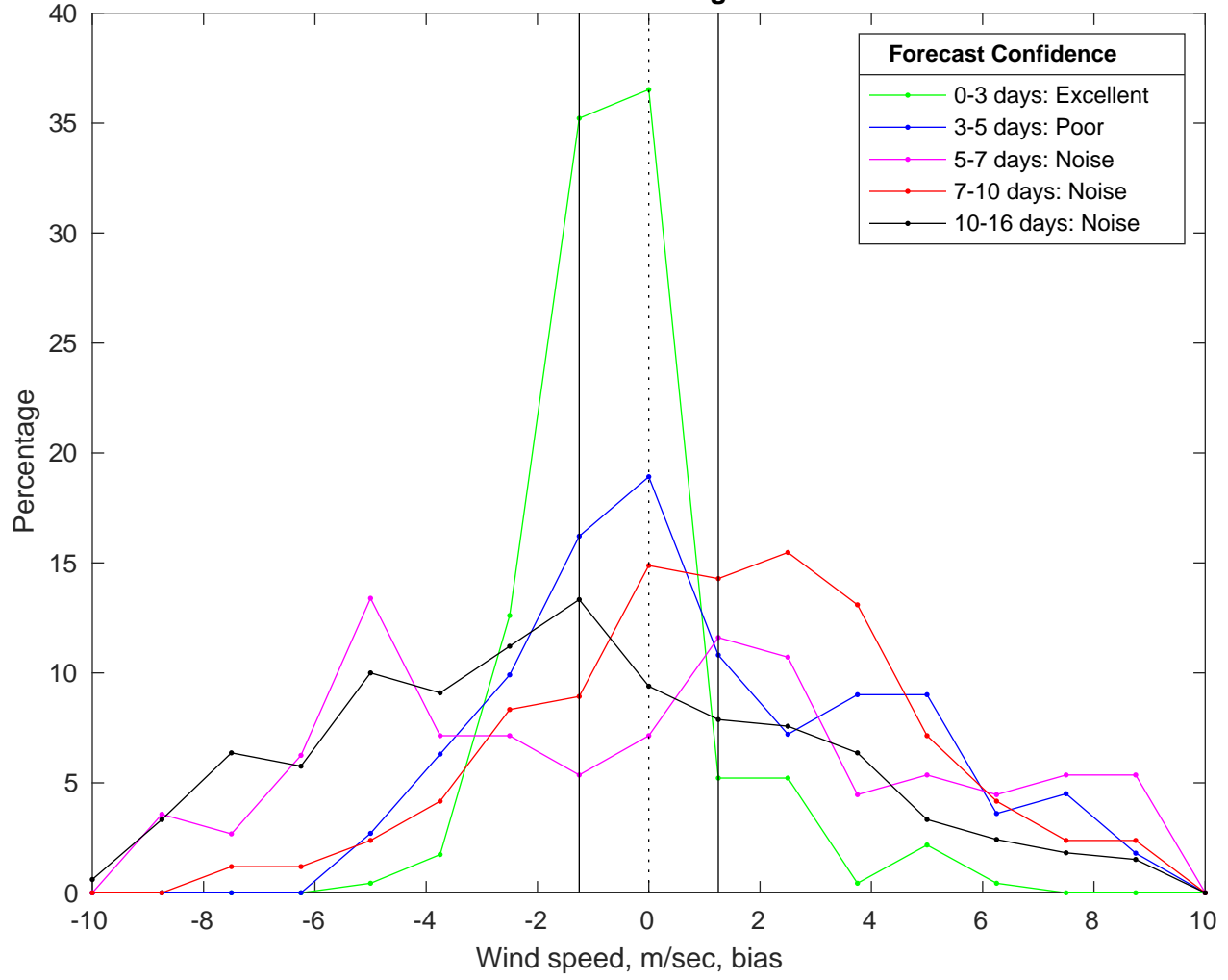
NDBC 42040 vs GFS Winds Bias Histogram: 24-Mar-2025
