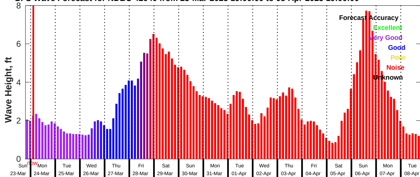
GFS Wave Forecast for NDBC 42040 from 23-Mar-2025 19:00:00 to 08-Apr-2025 19:00:00
