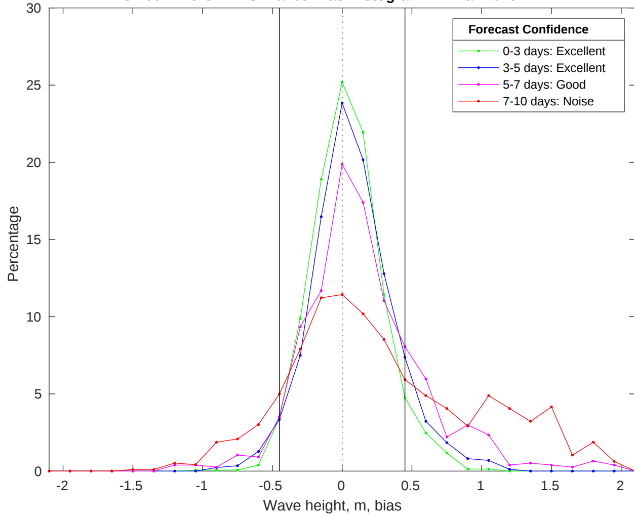
NDBC 46011 vs CMEMS Waves Bias Histogram: 24-Mar-2025
