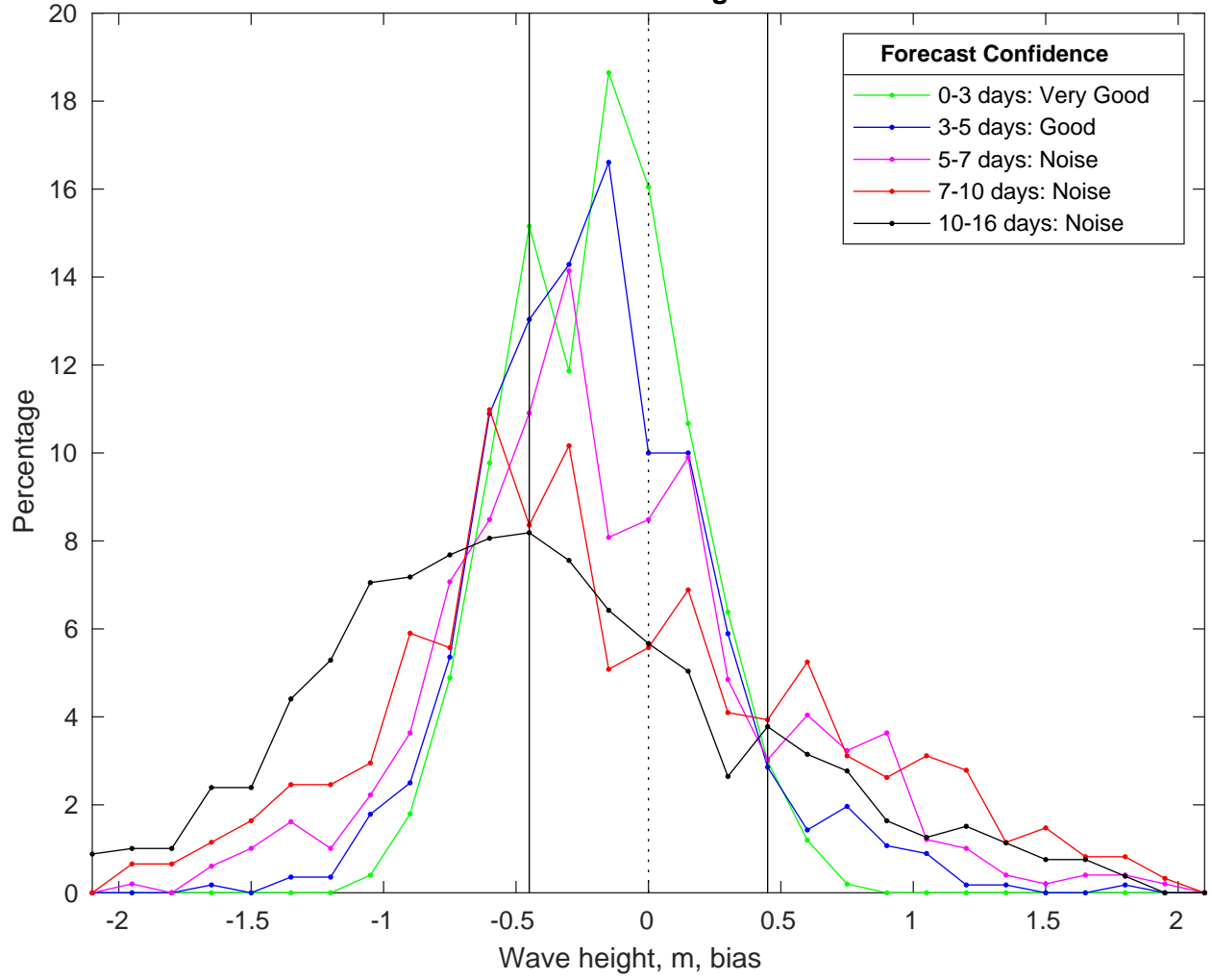
NDBC 46011 vs GFS Waves Bias Histogram: 24-Mar-2025
