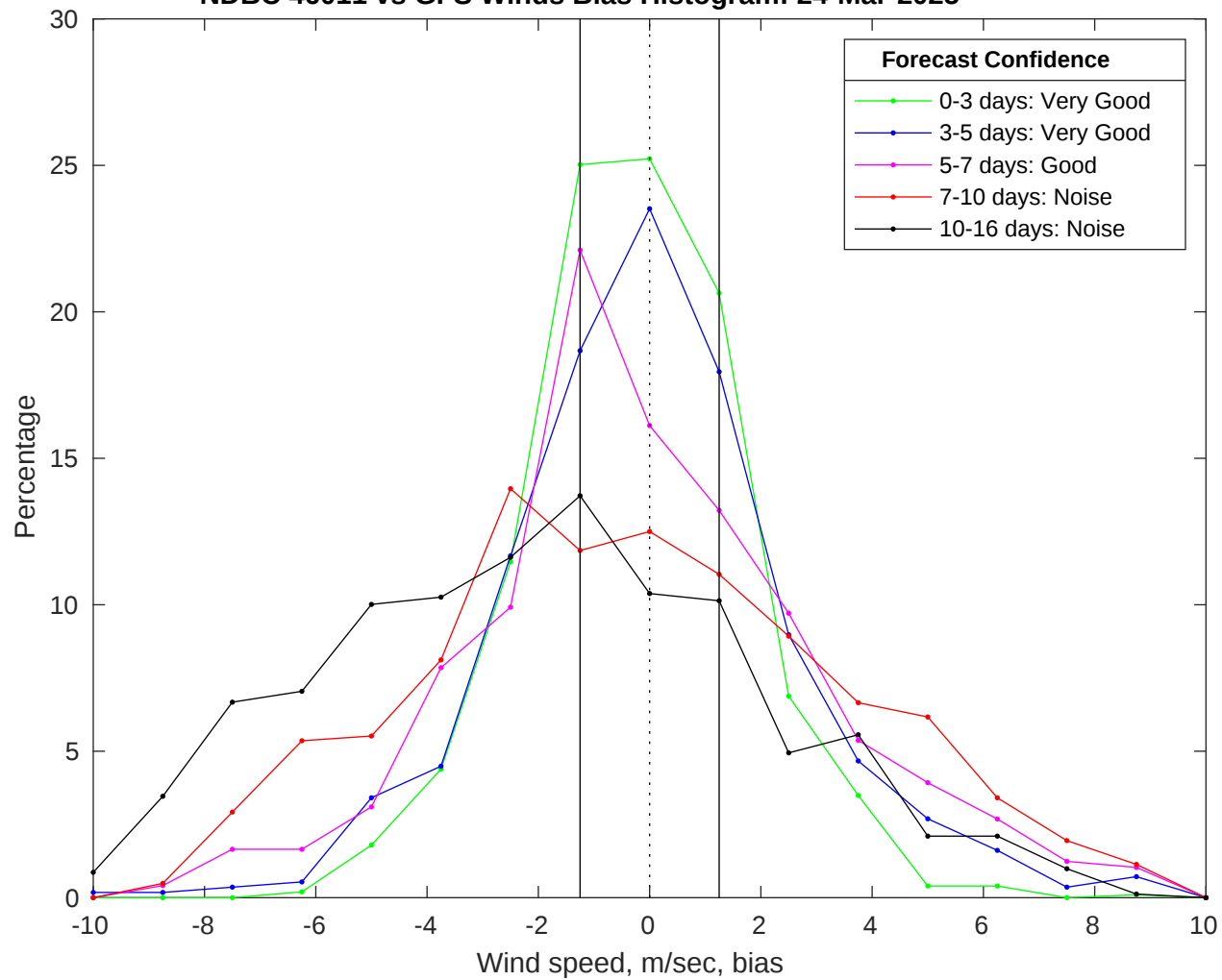
NDBC 46011 vs GFS Winds Bias Histogram: 24-Mar-2025
