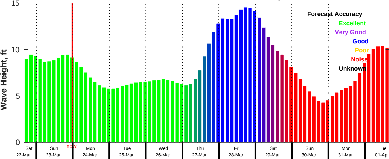
CMEMS Wave Forecast for NDBC 46011 from 22-Mar-2025 16:00:00 to 01-Apr-2025 16:00:00
