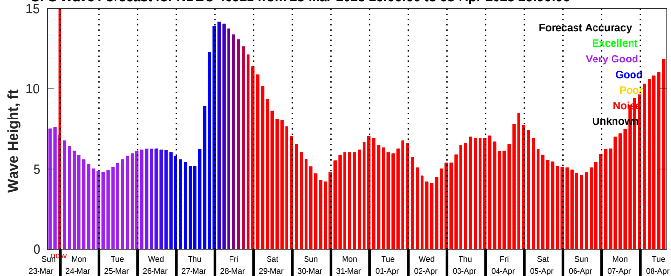
GFS Wave Forecast for NDBC 46011 from 23-Mar-2025 16:00:00 to 08-Apr-2025 16:00:00
