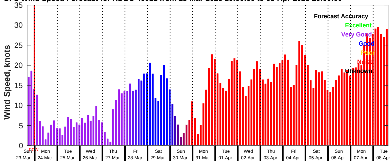
GFS Wind Speed Forecast for NDBC 46011 from 23-Mar-2025 16:00:00 to 08-Apr-2025 16:00:00
