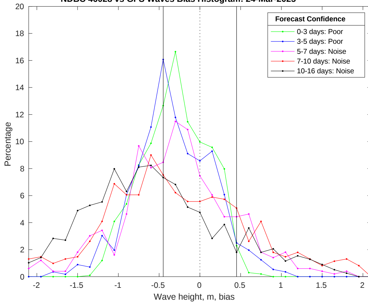
NDBC 46028 vs GFS Waves Bias Histogram: 24-Mar-2025
