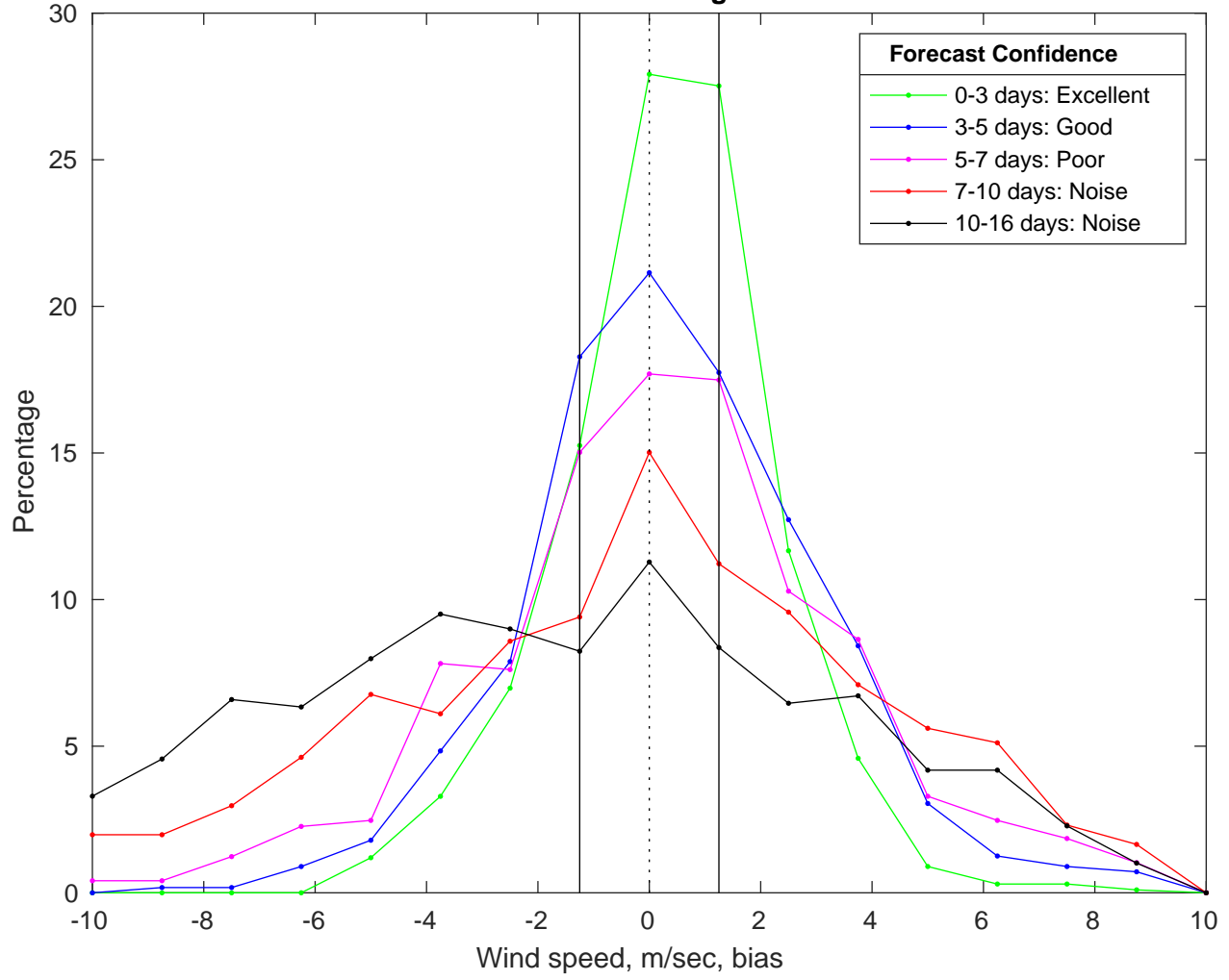
NDBC 46028 vs GFS Winds Bias Histogram: 24-Mar-2025
