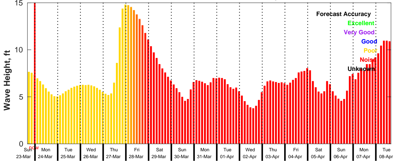
GFS Wave Forecast for NDBC 46028 from 23-Mar-2025 16:00:00 to 08-Apr-2025 16:00:00
