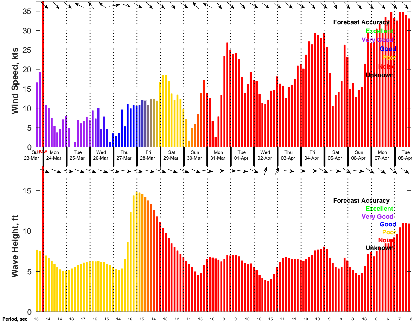
Wind & Wave Forecast for NDBC 46028 from 23-Mar-2025 16:00:00 to 08-Apr-2025 16:00:00
