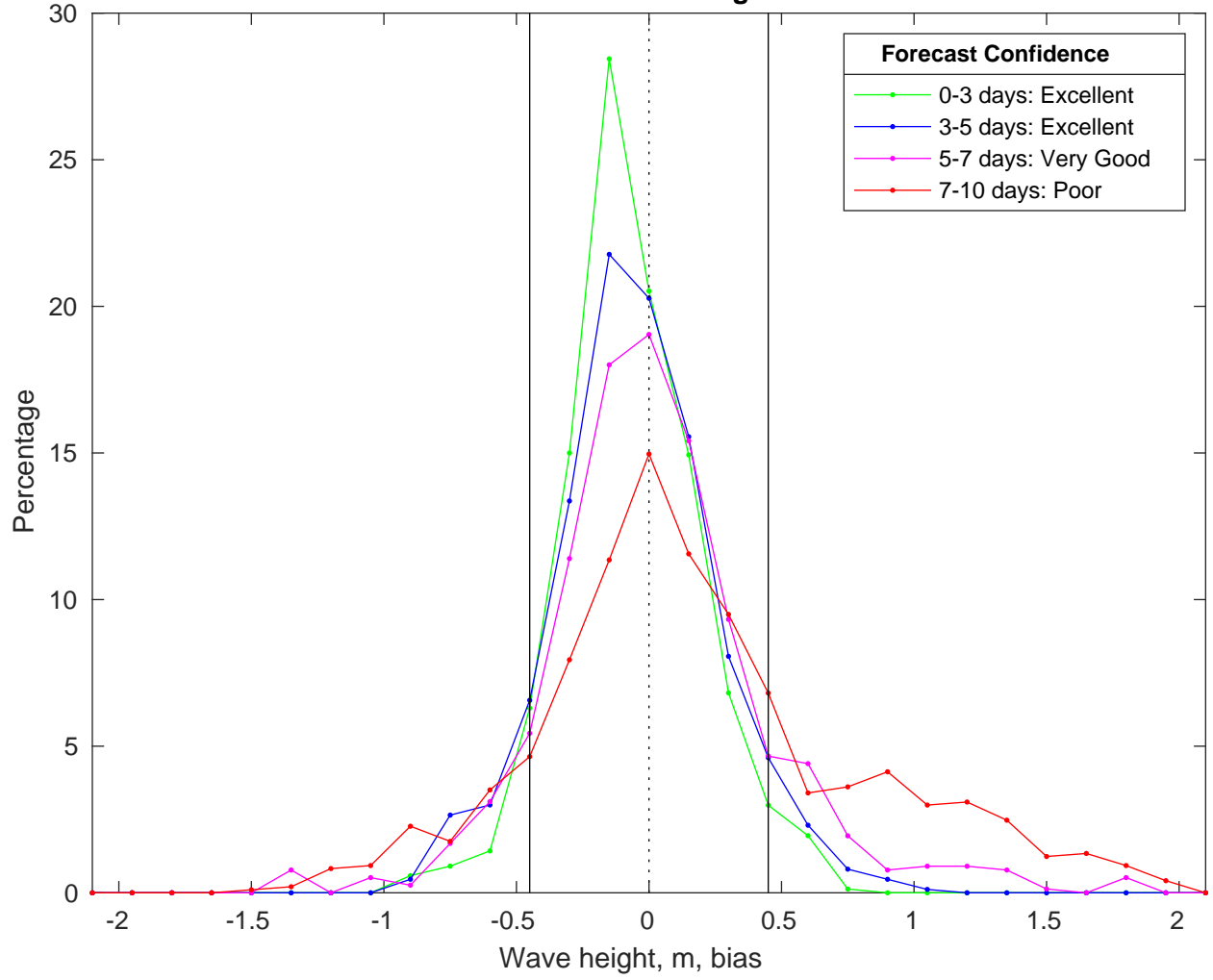
NDBC 46054 vs CMEMS Waves Bias Histogram: 24-Mar-2025
