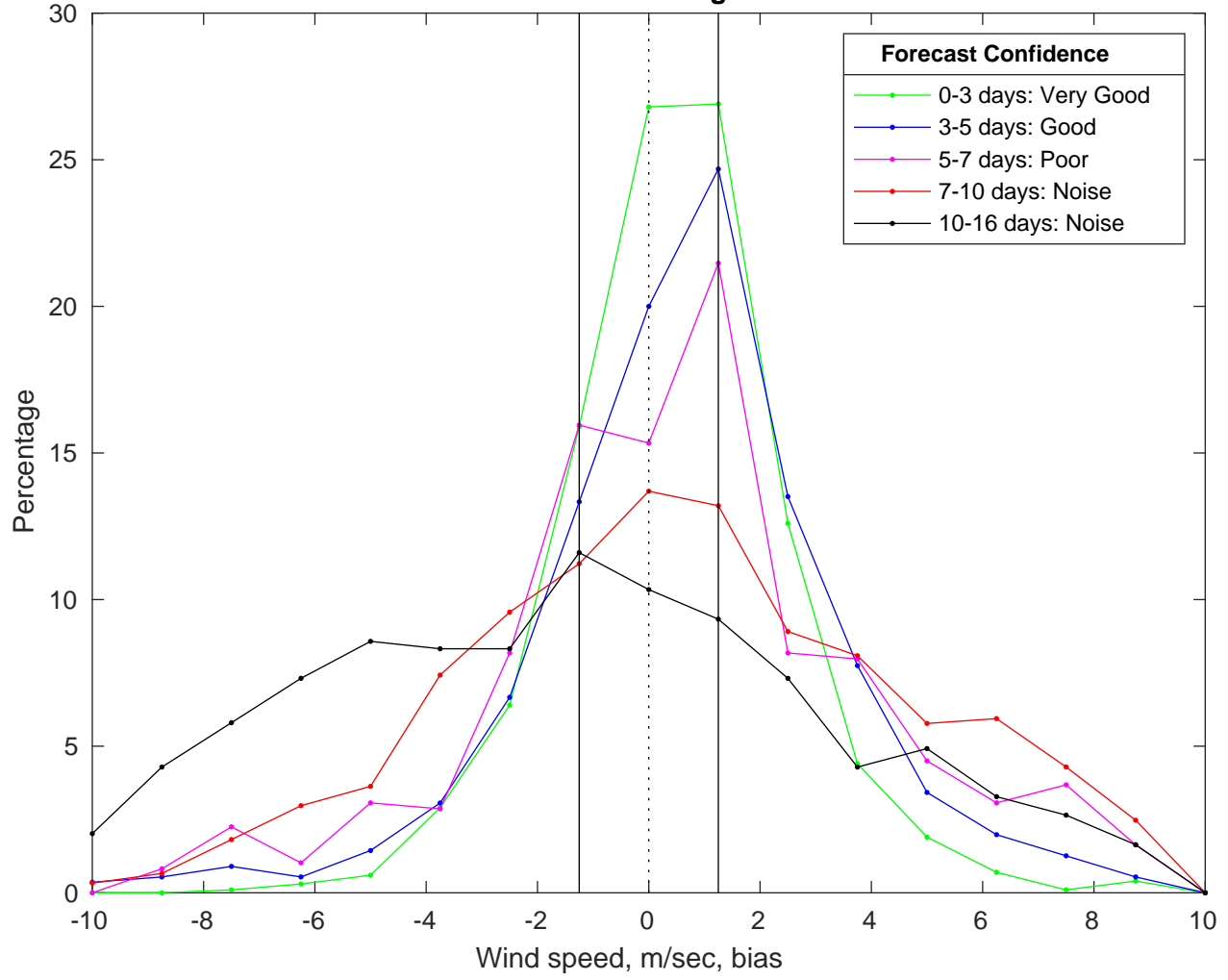
NDBC 46054 vs GFS Winds Bias Histogram: 24-Mar-2025
