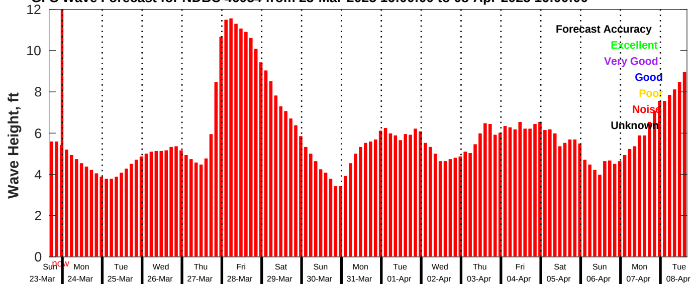
GFS Wave Forecast for NDBC 46054 from 23-Mar-2025 16:00:00 to 08-Apr-2025 16:00:00
