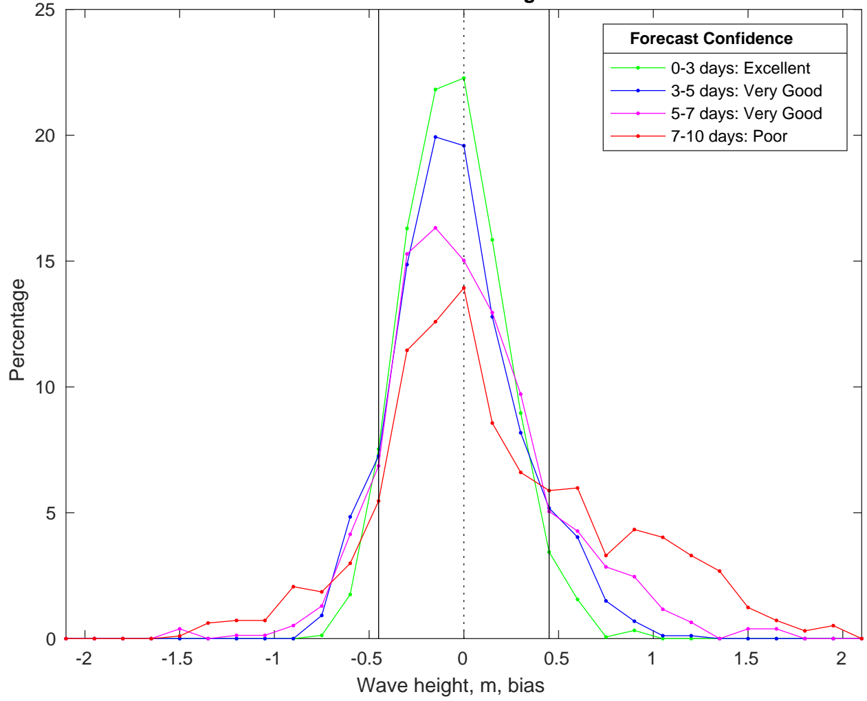
NDBC 46069 vs CMEMS Waves Bias Histogram: 24-Mar-2025
