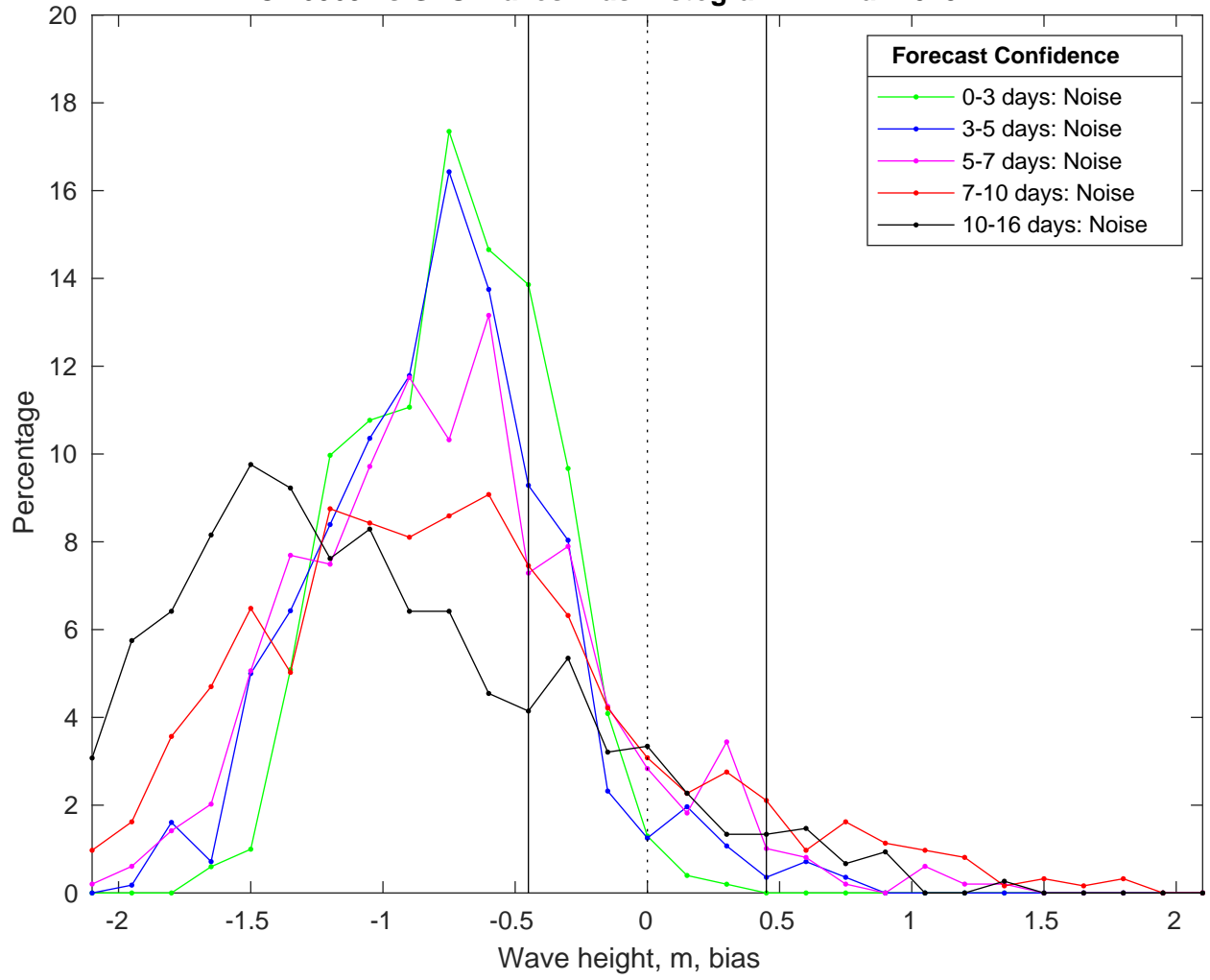
NDBC 46069 vs GFS Waves Bias Histogram: 24-Mar-2025
