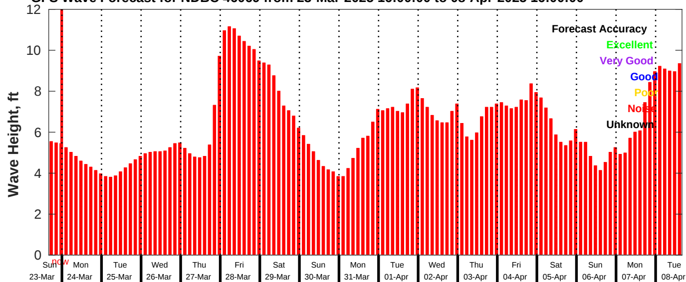
GFS Wave Forecast for NDBC 46069 from 23-Mar-2025 16:00:00 to 08-Apr-2025 16:00:00
