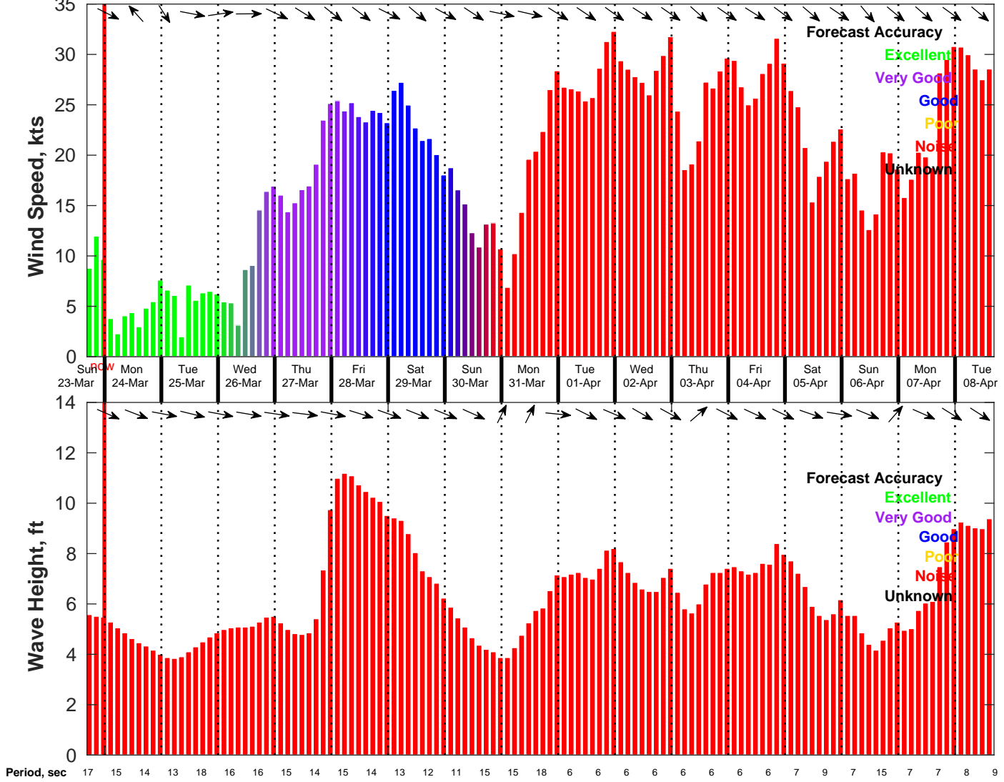
Wind & Wave Forecast for NDBC 46069 from 23-Mar-2025 16:00:00 to 08-Apr-2025 16:00:00
