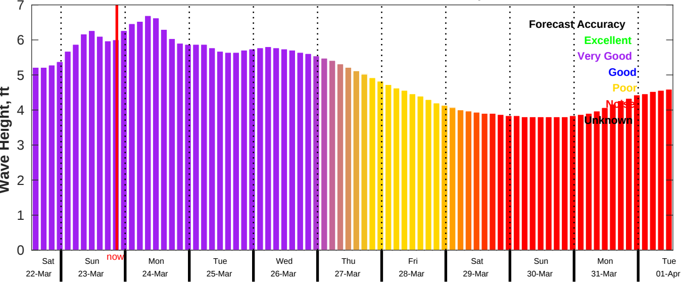
CMEMS Wave Forecast for NDBC 51209 from 22-Mar-2025 13:00:00 to 01-Apr-2025 13:00:00
