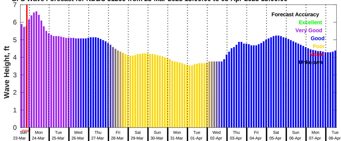
GFS Wave Forecast for NDBC 51209 from 23-Mar-2025 13:00:00 to 08-Apr-2025 13:00:00
