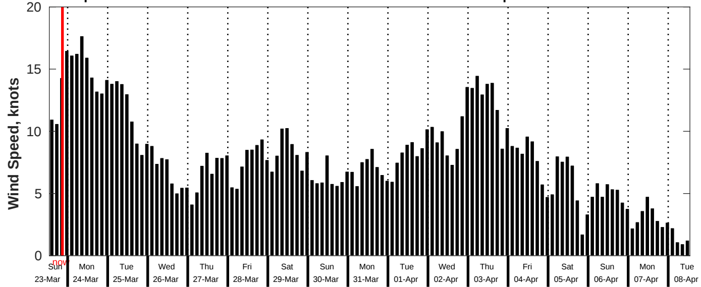
GFS Wind Speed Forecast for NDBC 51209 from 23-Mar-2025 13:00:00 to 08-Apr-2025 13:00:00
