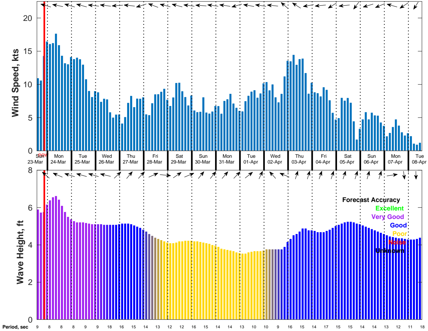
Wind & Wave Forecast for NDBC 51209 from 23-Mar-2025 13:00:00 to 08-Apr-2025 13:00:00
