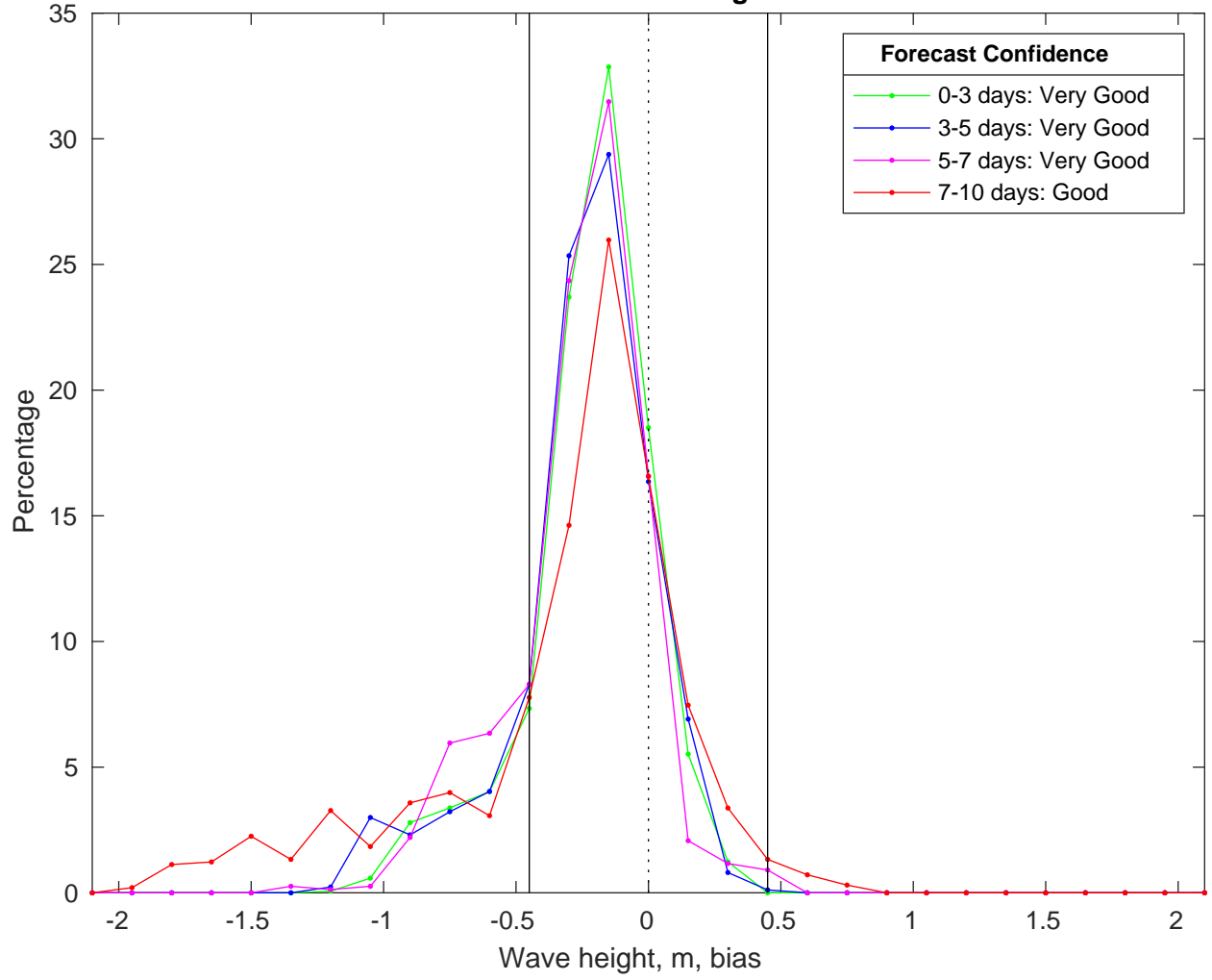
NDBC 52211 vs CMEMS Waves Bias Histogram: 24-Mar-2025
