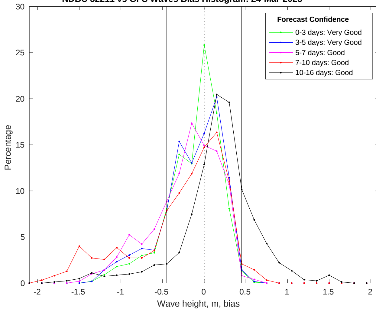
NDBC 52211 vs GFS Waves Bias Histogram: 24-Mar-2025
