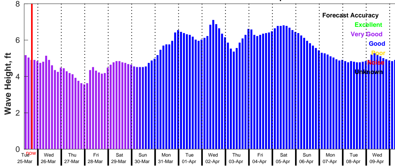
GFS Wave Forecast for NDBC 52211 from 24-Mar-2025 10:00:00 to 09-Apr-2025 10:00:00
