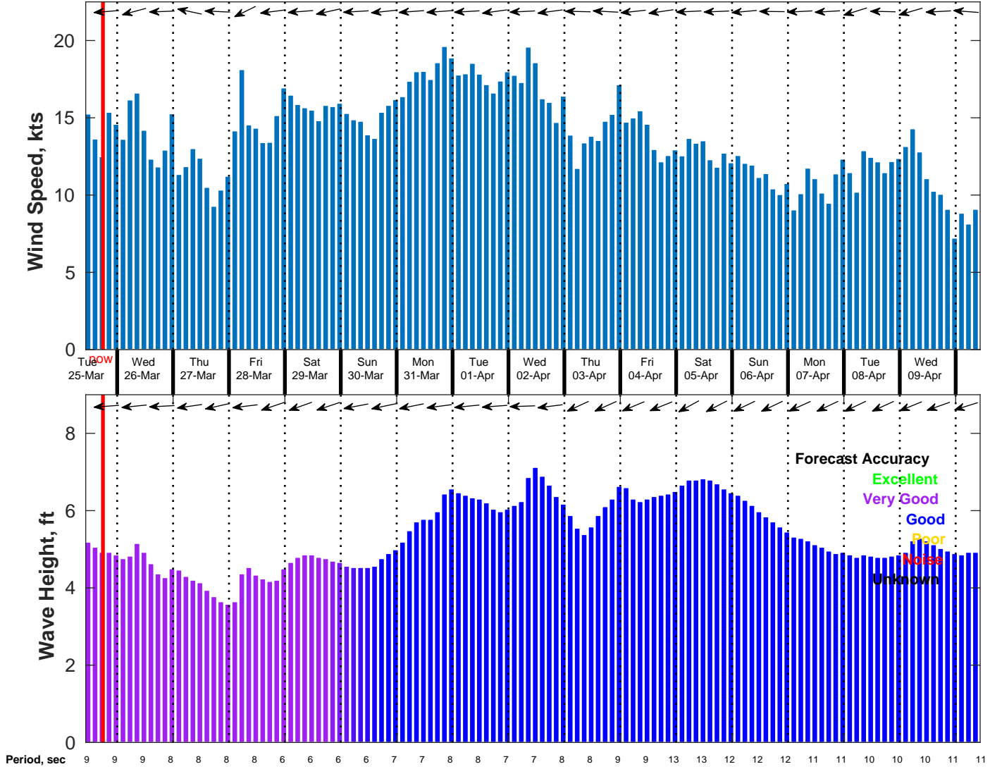
Wind & Wave Forecast for NDBC 52211 from 24-Mar-2025 10:00:00 to 09-Apr-2025 10:00:00
