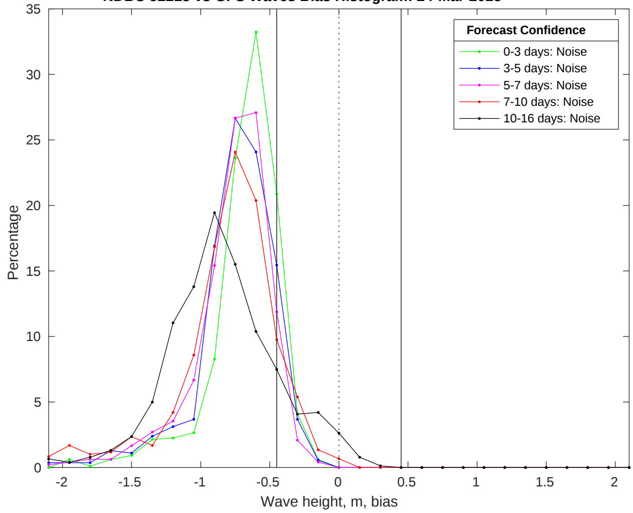
NDBC 52213 vs GFS Waves Bias Histogram: 24-Mar-2025
