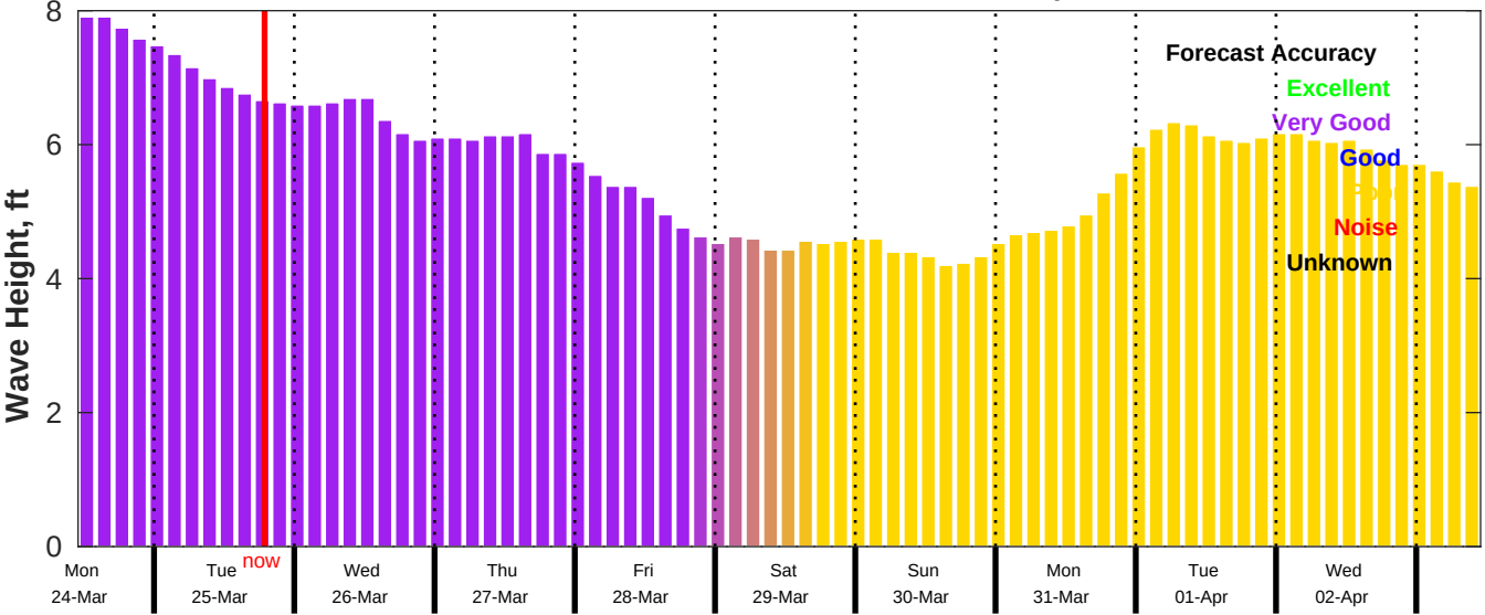
CMEMS Wave Forecast for NDBC 52213 from 23-Mar-2025 11:00:00 to 02-Apr-2025 11:00:00
