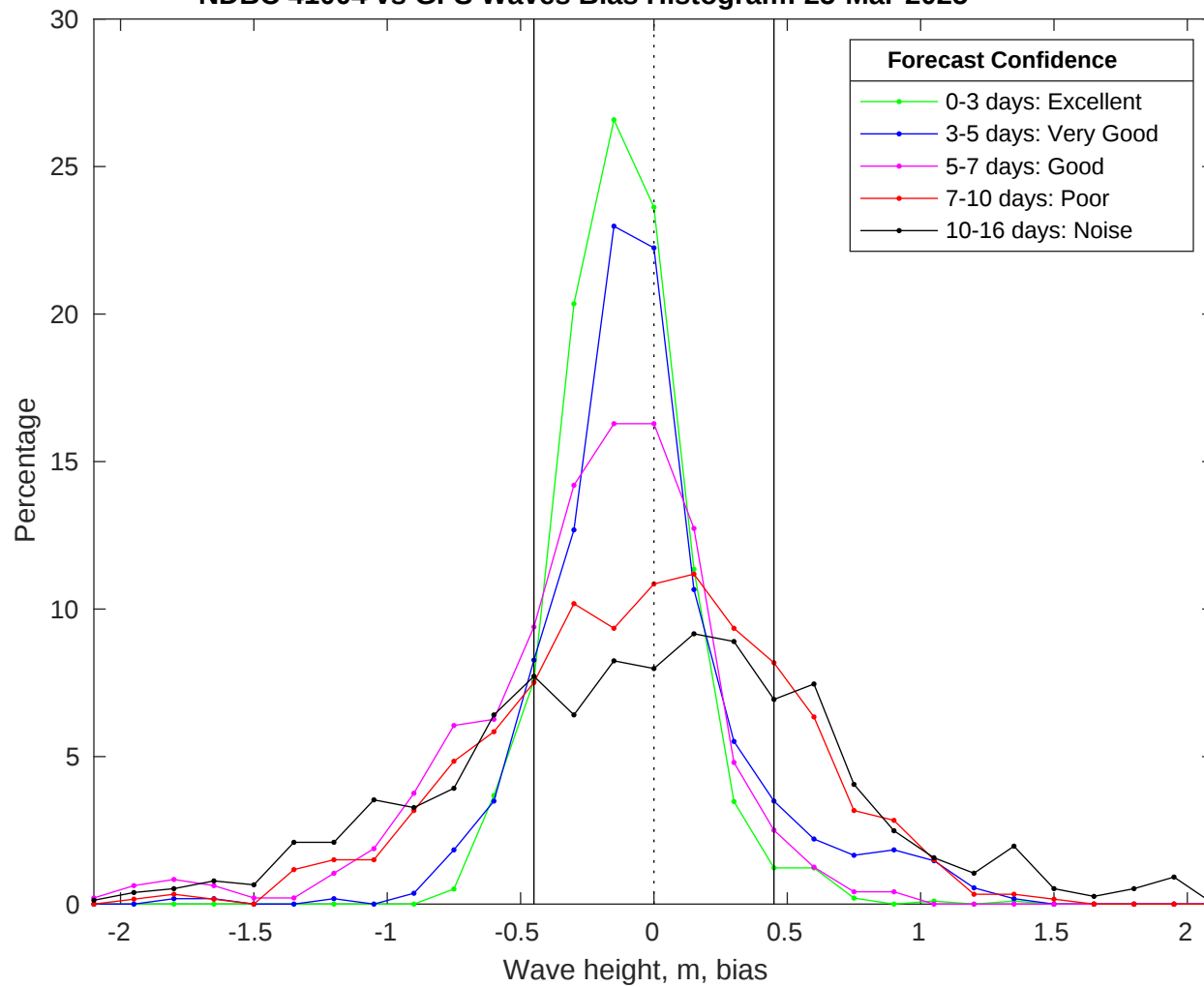
NDBC 41004 vs GFS Waves Bias Histogram: 25-Mar-2025
