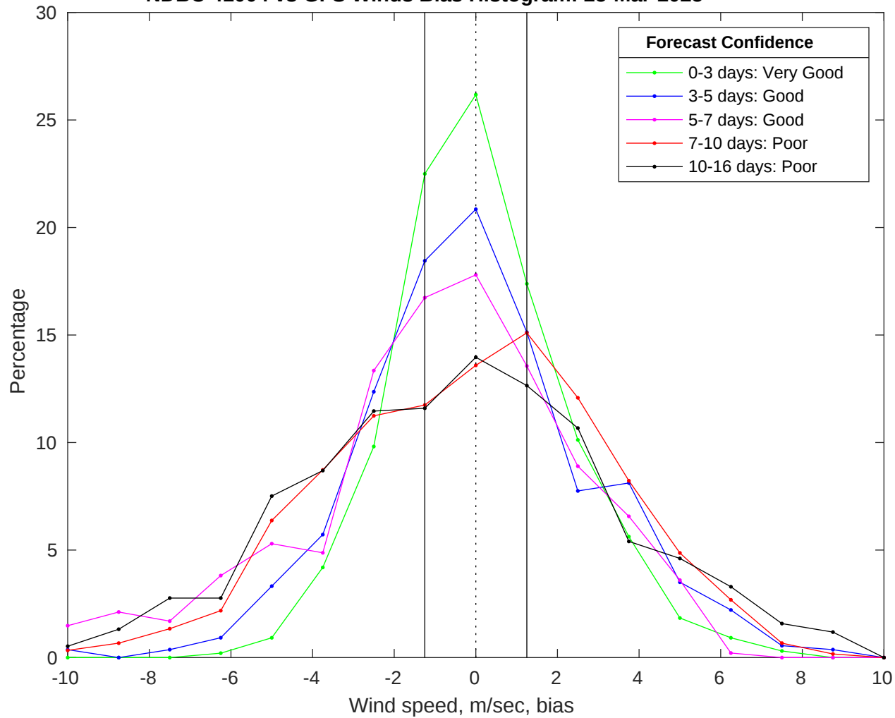
NDBC 41004 vs GFS Winds Bias Histogram: 25-Mar-2025
