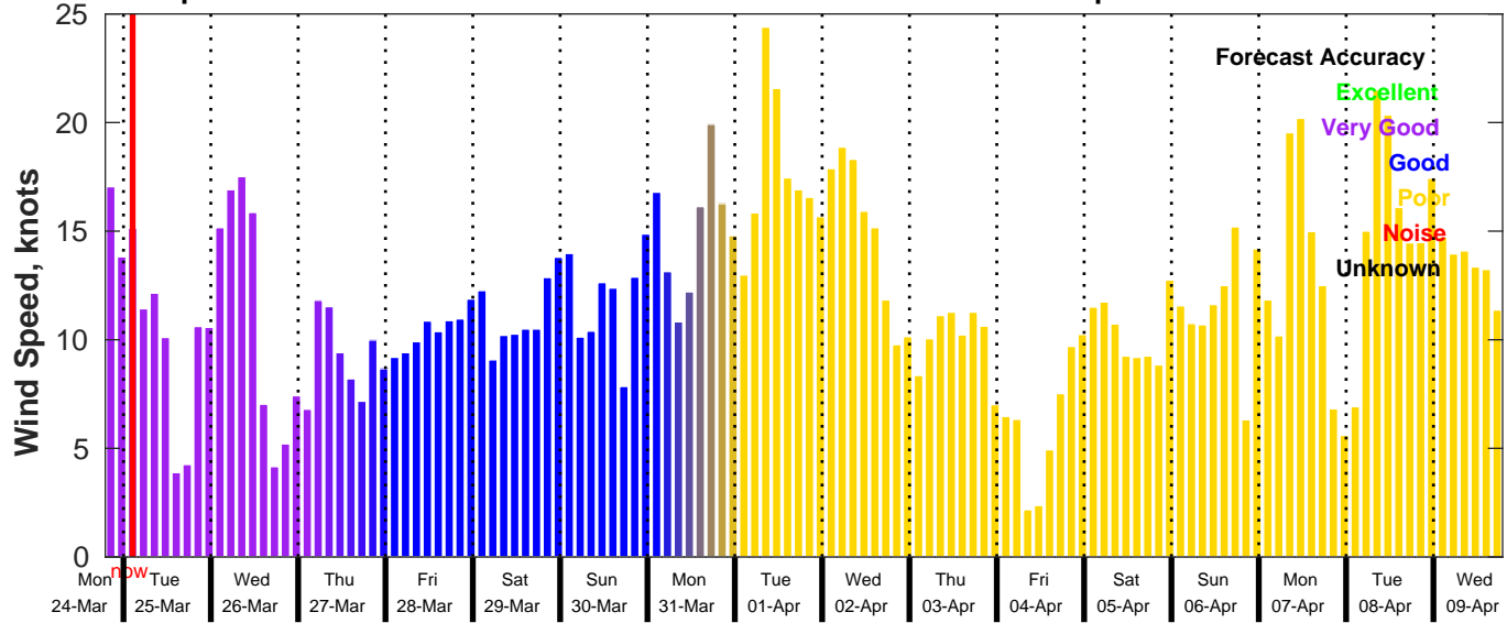
GFS Wind Speed Forecast for NDBC 41004 from 24-Mar-2025 19:00:00 to 09-Apr-2025 19:00:00
