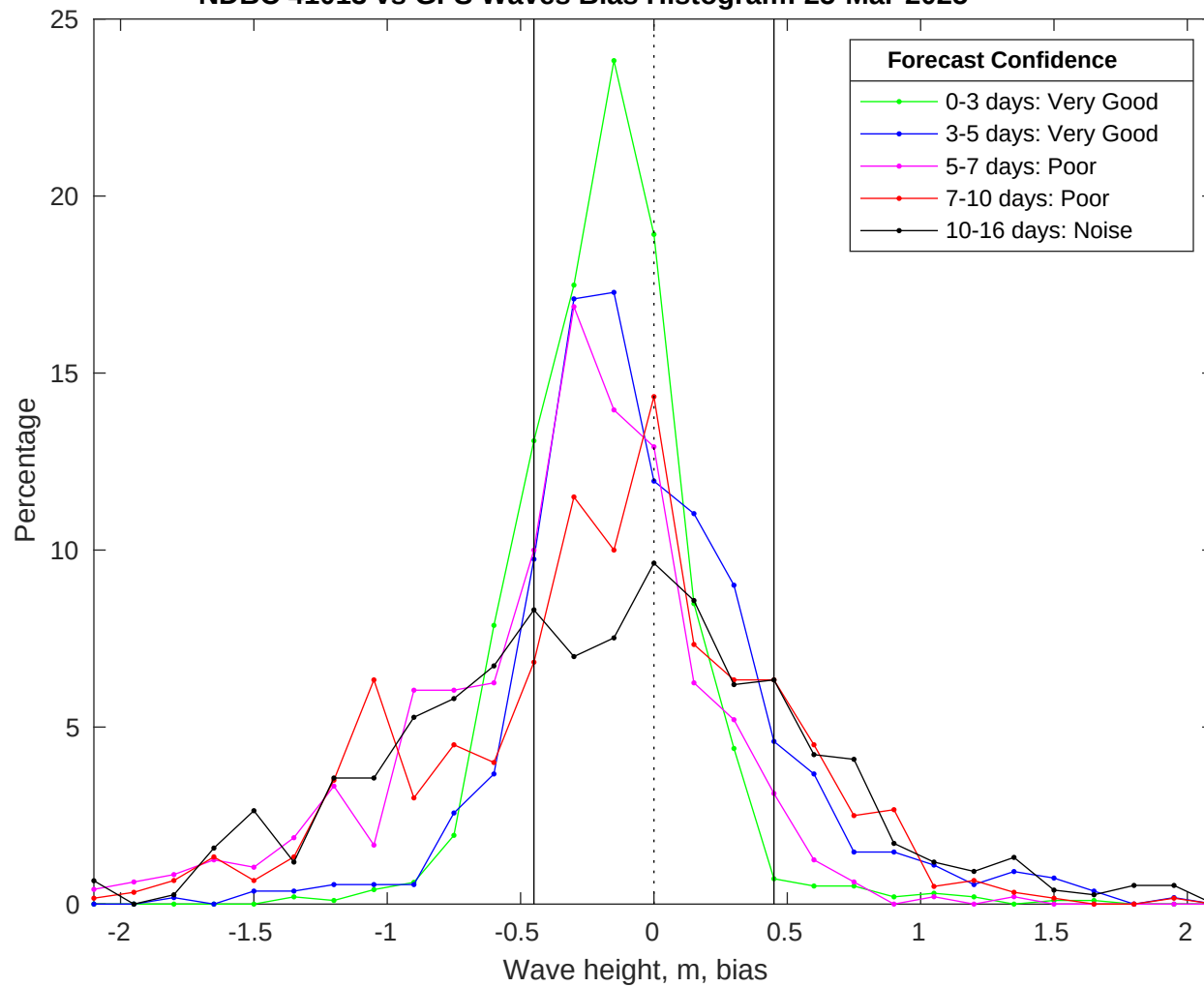
NDBC 41013 vs GFS Waves Bias Histogram: 25-Mar-2025
