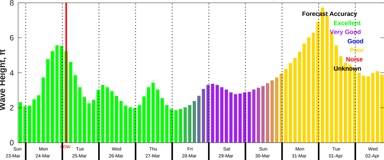
CMEMS Wave Forecast for NDBC 41013 from 23-Mar-2025 19:00:00 to 02-Apr-2025 19:00:00
